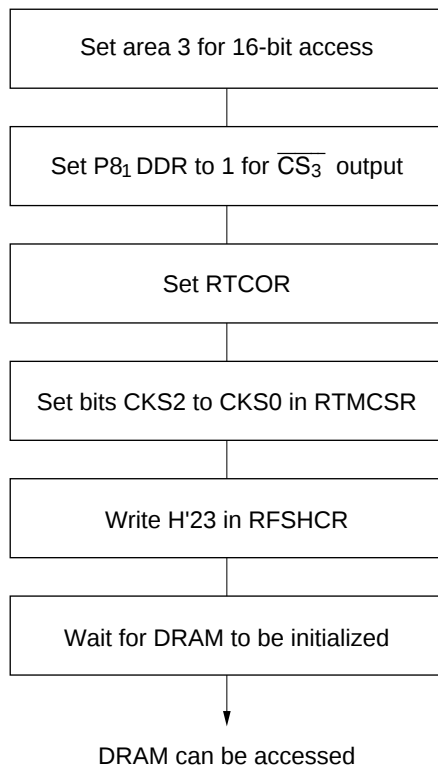
Figure 7-10 Setup Procedure for 2\overline{\text{WE}} 4-Mbit DRAM with 10-Bit Row Address and 8-Bit Column Address (16-Mbyte Mode)
