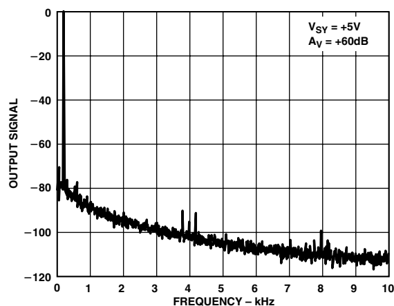
Figure 53b. Spectral Analysis Using a Feedback Capacitor
