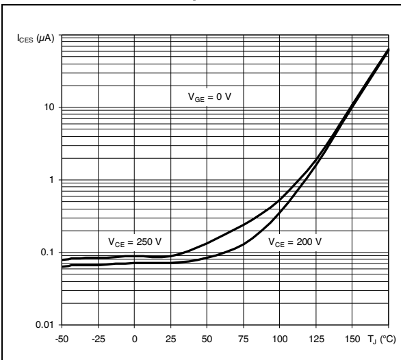
Figure 8. Collector cut-off current vs temperature
