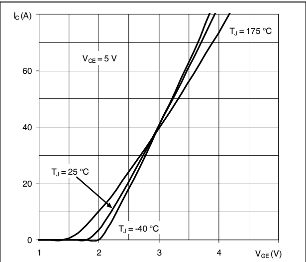
Figure 7. Transfer characteristics
