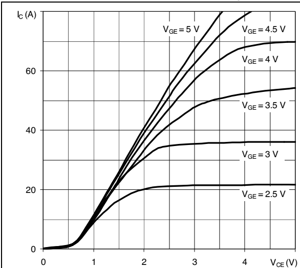
Figure 6. Output characteristics ( T_J = 175\text{ }^{\circ}\text{C} )
