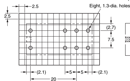
PCB Mounting Holes (BOTTOM VIEW) Tolerance: \pm 0.1 mm
