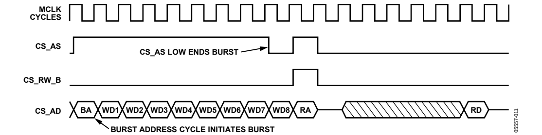
Figure 17. Write Burst Mode Functional Timing
