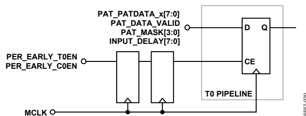
Figure 9. PER_EARLY_T0EN Pipelining
