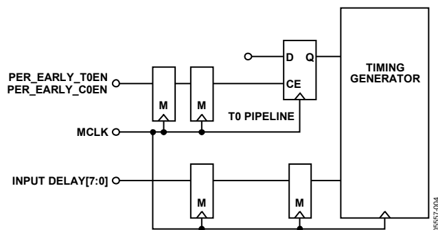
Figure 10. INPUT_DELAY Pipeline
