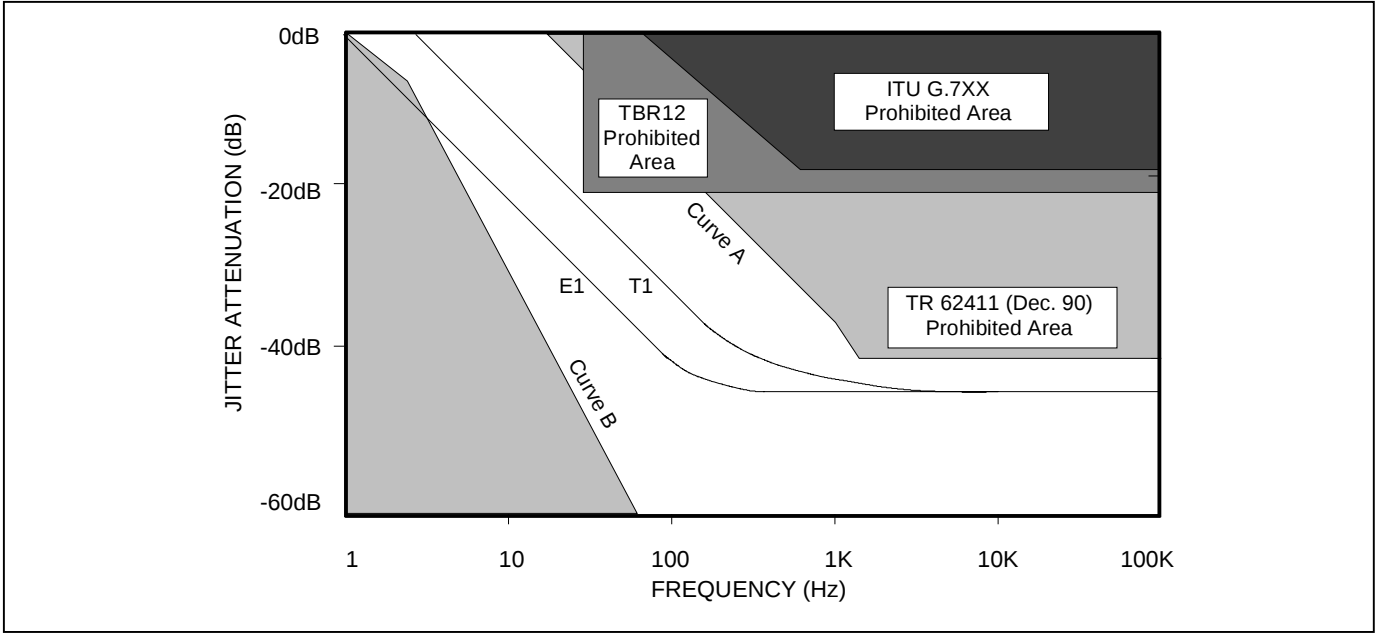
Figure 9-26. Jitter Attenuation
