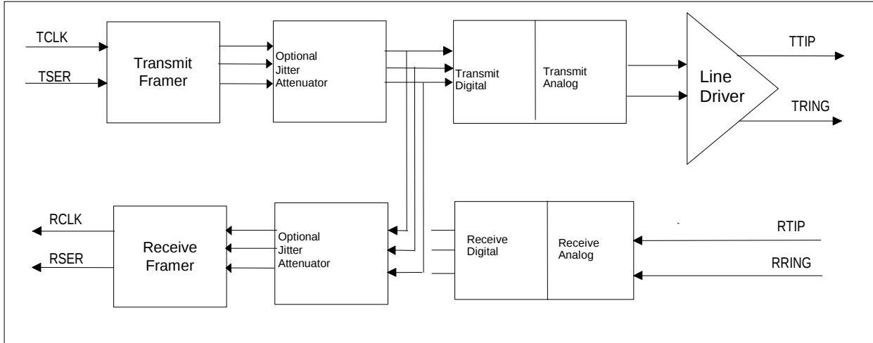
Figure 9-29. Local Loopback
