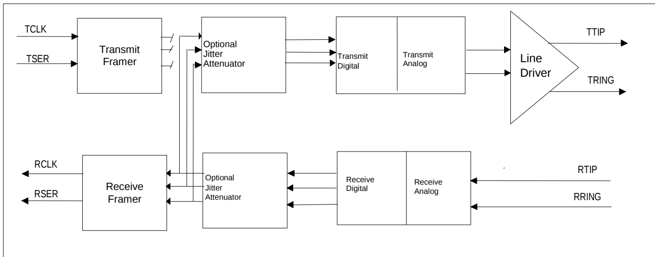
Figure 9-30. Remote Loopback 2
