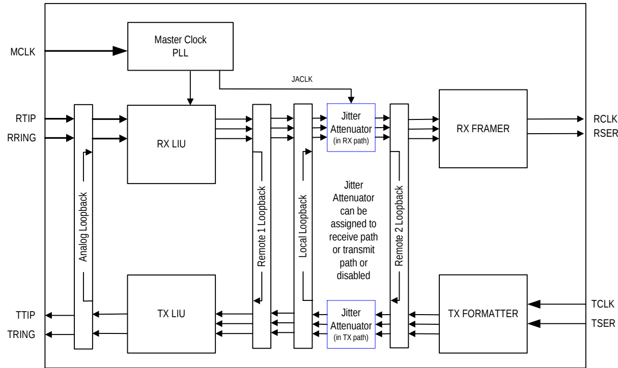
Figure 9-27. Loopback Diagram
