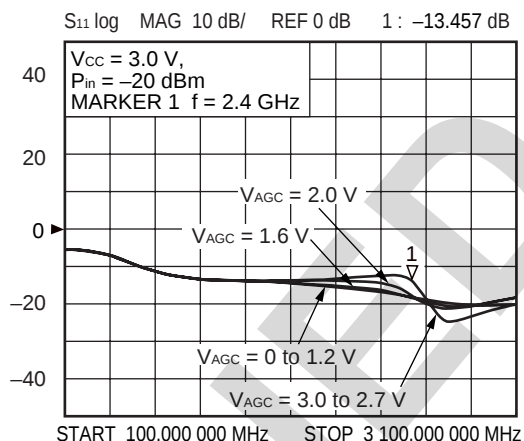
S 11 —FREQUENCY
