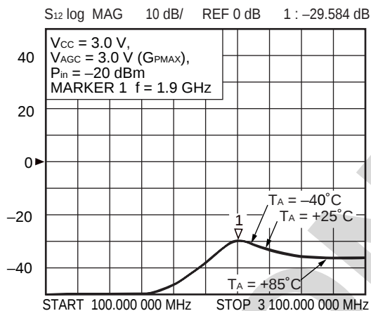
S 12 —FREQUENCY
