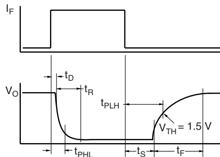
Fig. 13 - Switching Timing
