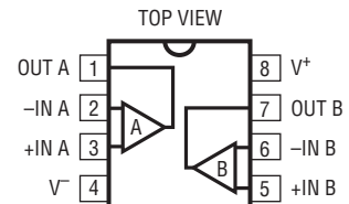
N8 PACKAGE 8-LEAD PDIP
