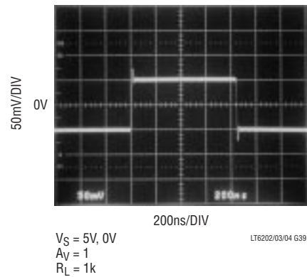
5V Small-Signal Response
