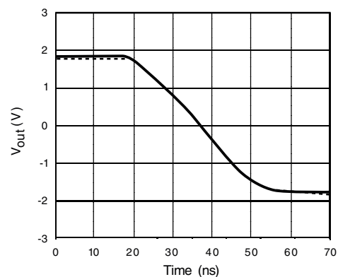
Figure 7. Large signal measurement – negative slew rate ( V_{CC} = \pm 2.5 V) Gain = +2, Z_L = 150\ \Omega // 5.6\ \text{pF} , V_{in} = 400\ \text{mVpk}
