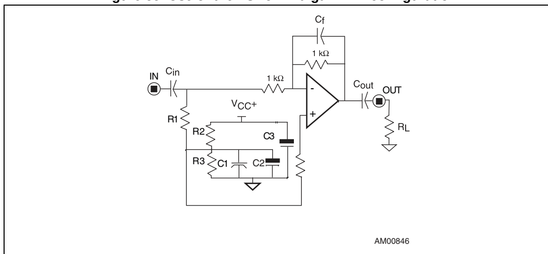
Figure 35. Use of the TSH8x in a gain = -1 configuration
