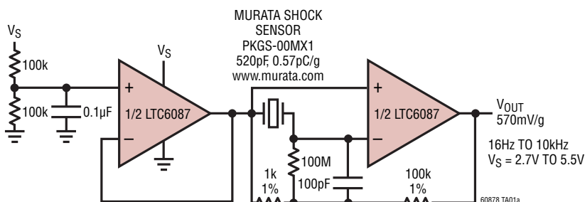
Single Supply Shock/Vibration Sensor Amplifier
