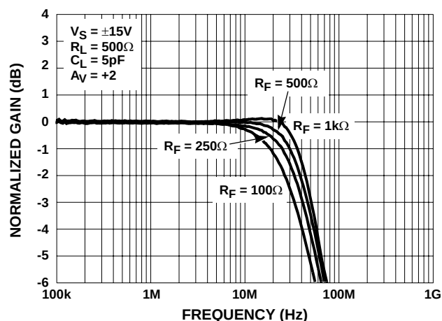
FIGURE 14. GAIN vs FREQUENCY FOR VARIOUS R_{FEEDBACK} ( A_V = +2 )
