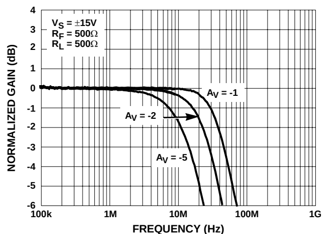
FIGURE 4. GAIN vs FREQUENCY FOR VARIOUS INVERTING GAIN SETTINGS
