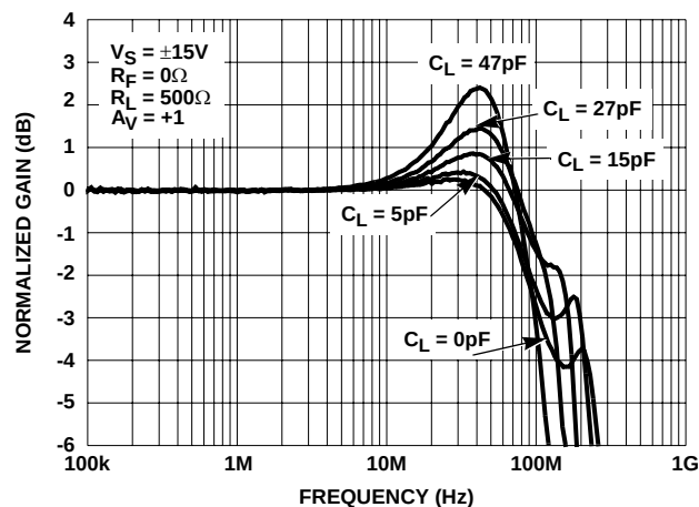
FIGURE 11. GAIN vs FREQUENCY FOR VARIOUS C_{LOAD} ( A_V = +1 )
