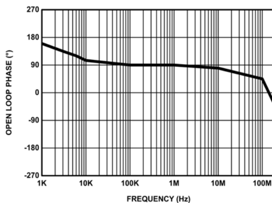
FIGURE 2. OPEN-LOOP PHASE vs FREQUENCY
