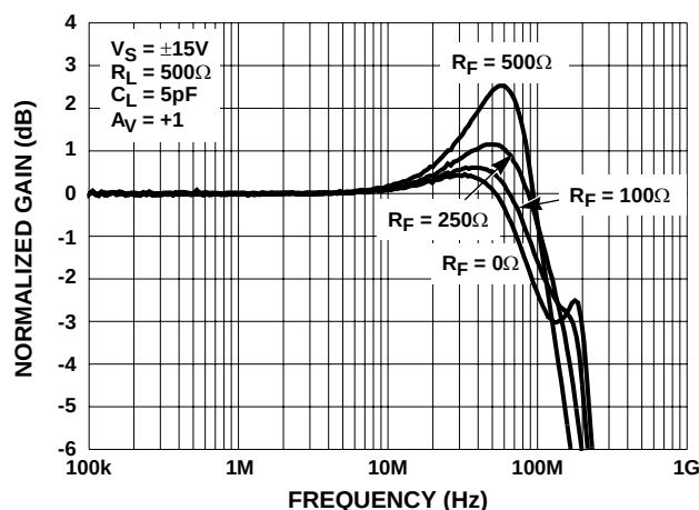
FIGURE 13. GAIN vs FREQUENCY FOR VARIOUS R_{FEEDBACK} ( A_V = +1 )
