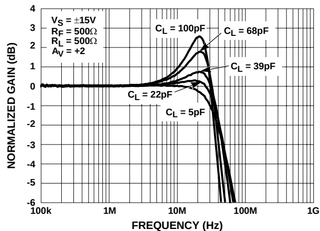
FIGURE 12. GAIN vs FREQUENCY FOR VARIOUS C_{LOAD} ( A_V = +2 )
