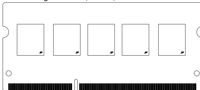
Figure 1: 204-Pin SODIMM (MO-268 R/C C1)
