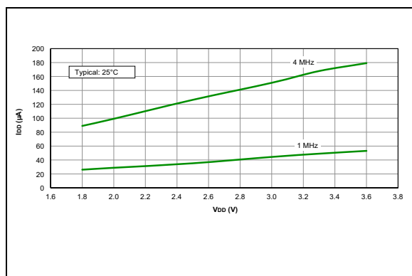
FIGURE 26-2: I_{DD} Typical, EC Oscillator, Medium-Power Mode
