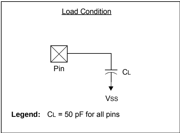
FIGURE 25-3: LOAD CONDITIONS
