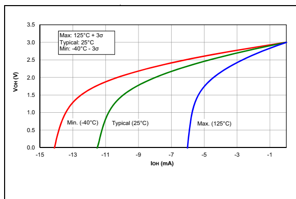
FIGURE 26-14: VOH vs. IOH , over Temperature, V_{DD}=3.0V
