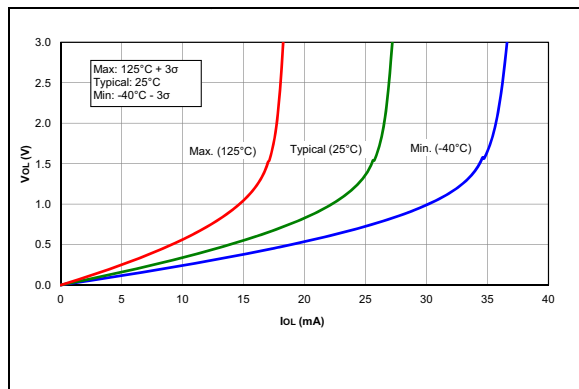
FIGURE 26-15: VOL vs. IOL , over Temperature, V_{DD}=3.0V
