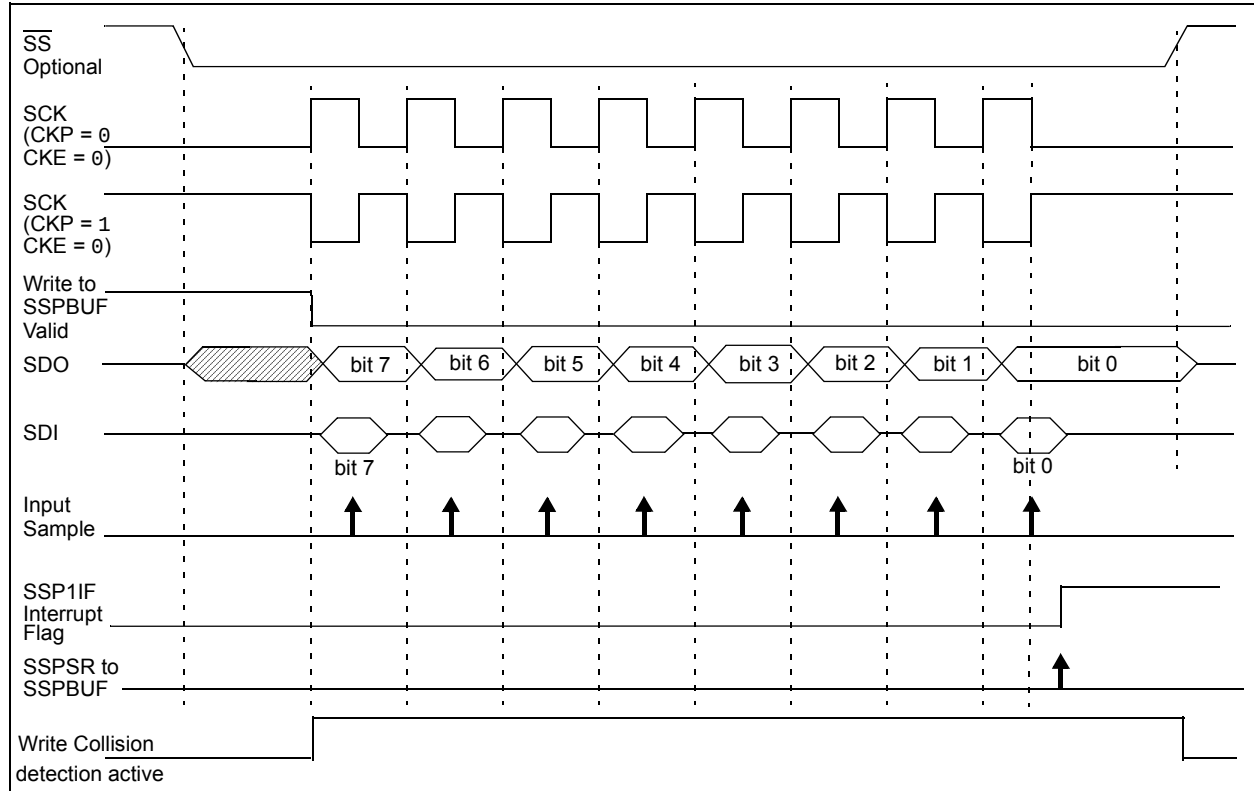
FIGURE 20-9: SPI MODE WAVEFORM (SLAVE MODE WITH CKE = 0)
