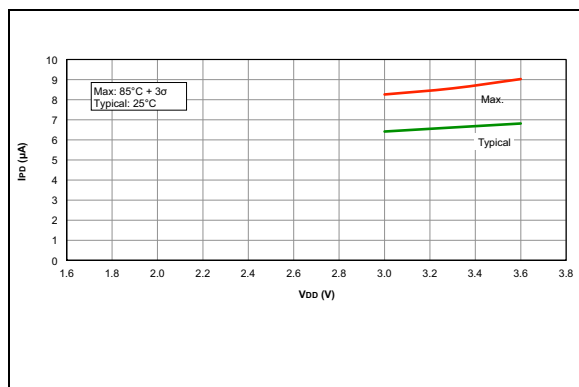
FIGURE 26-13: IPD , Brown-out Reset (BOR)
