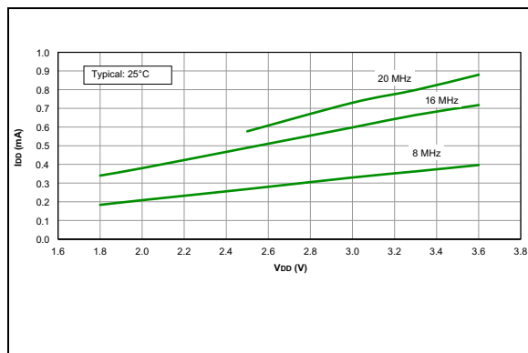
FIGURE 26-3: I_{DD} Typical, EC Oscillator, High-Power Mode
