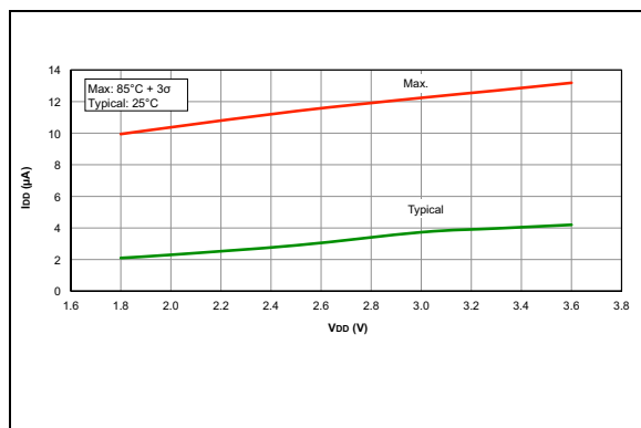
FIGURE 26-1: I_{DD} , EC Oscillator, Low-Power mode, F_{osc}=32 kHz
