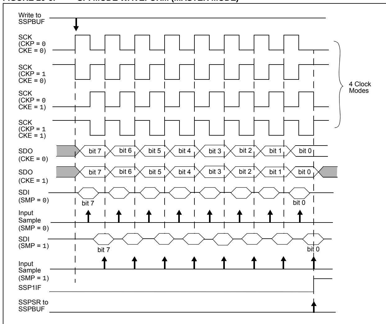
FIGURE 20-6: SPI MODE WAVEFORM (MASTER MODE)
