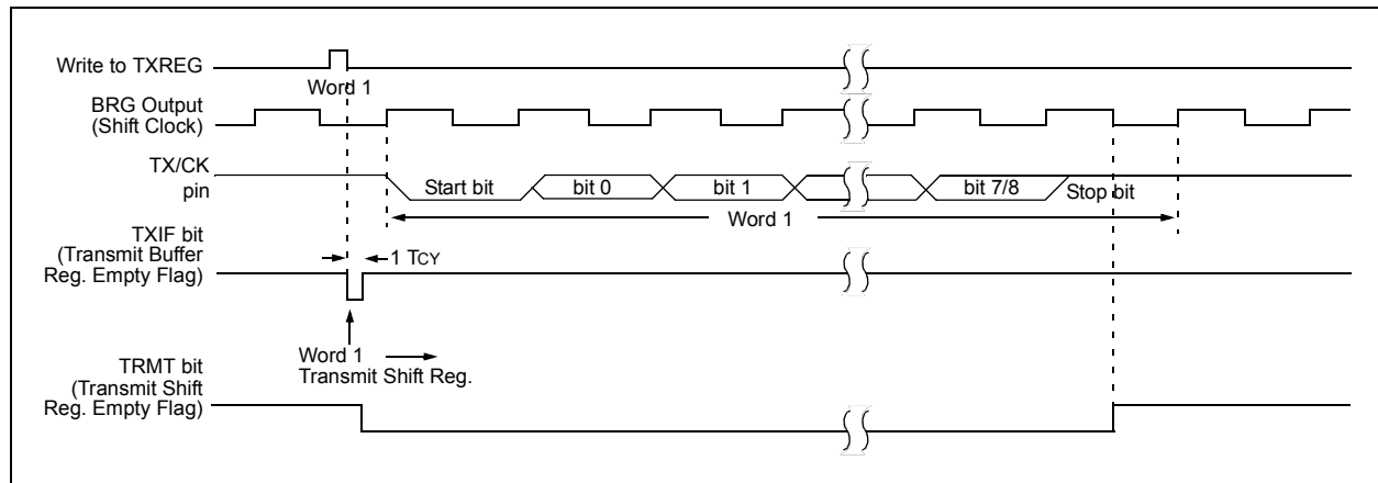
FIGURE 21-3: ASYNCHRONOUS TRANSMISSION
