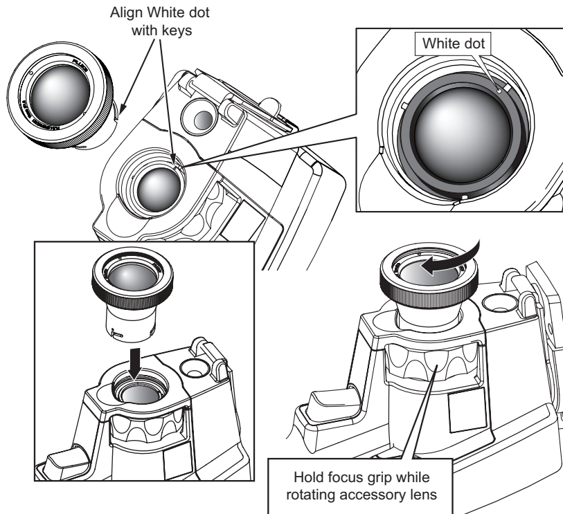
Figure 1. Attachment and Removal of Optional Lenses
