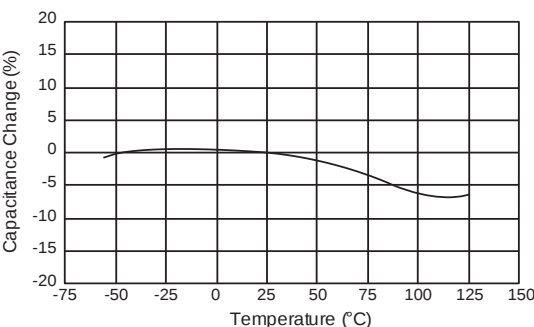
[Example of Temperature Caracteristics X7R(R7)] Sample: 0.1μF, Rated Voltage 50VDC
