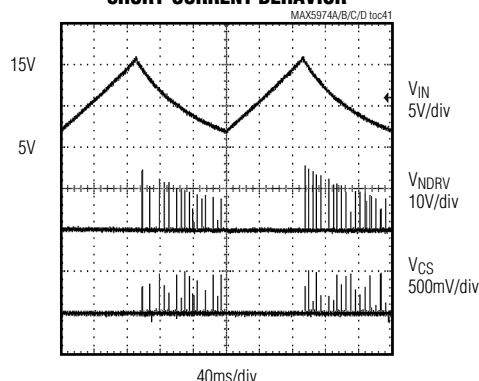
SHORT-CURRENT BEHAVIOR
