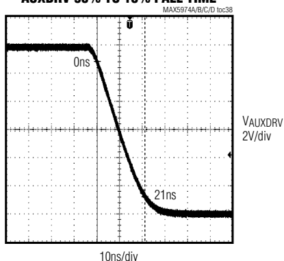
AUXDRV 90% TO 10% FALL TIME
