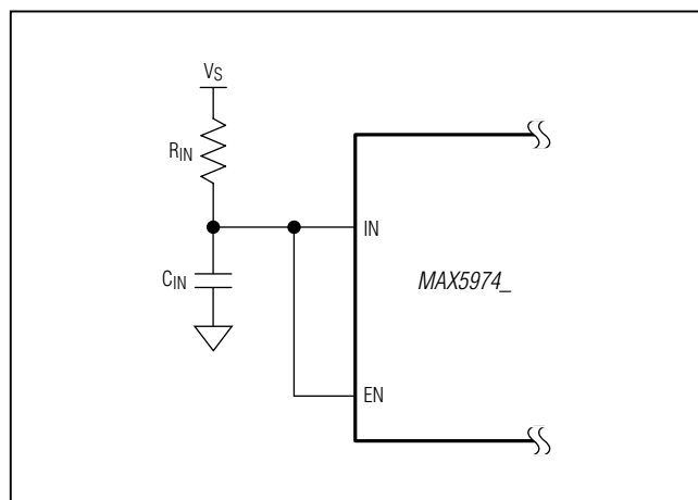
Figure 4. Always-On Operation
