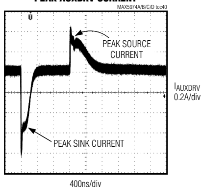
PEAK AUXDRV CURRENT
