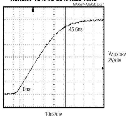
AUXDRV 10% TO 90% RISE TIME
