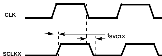
FIGURE 24. SCLKX OUTPUT TIMING IN 1X MODE
