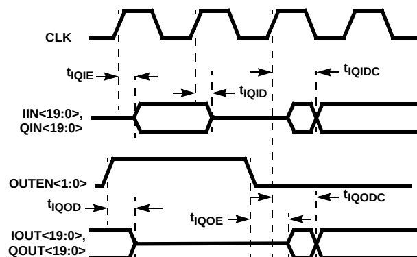
FIGURE 22. ENABLE/DISABLE TIMING
