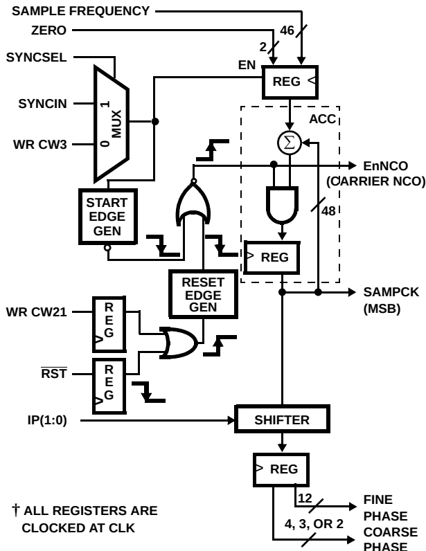
FIGURE 11. RE-SAMPLING NCO BLOCK DIAGRAM
