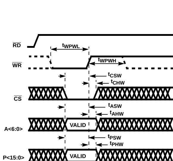
FIGURE 25. MICROPROCESSOR WRITE TIMING (RDmode = 0)
