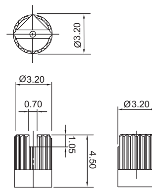
C: KNURLED, SLOTTED SHAFT
