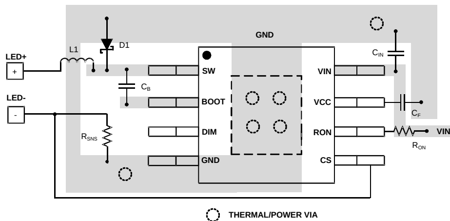
Figure 34. Layout Example
