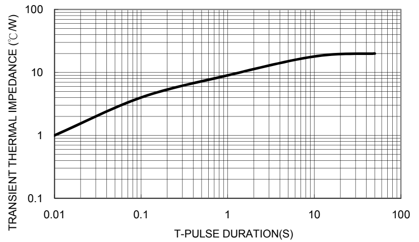
FIG. 6 TYPICAL TRANSIENT THERMAL IMPEDANCE
