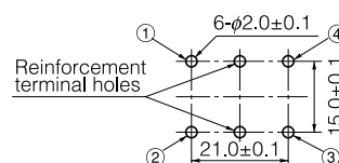
Recommended PWB piercing plan
