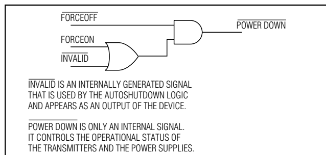
Figure 3c. MAX32x_E AutoShutdown Logic
