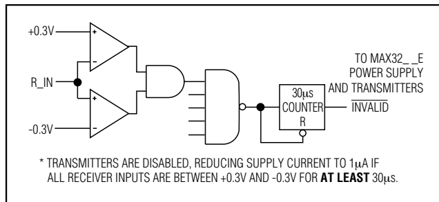
Figure 3a. MAX32_E Entering 1μA Supply Mode via AutoShutdown
