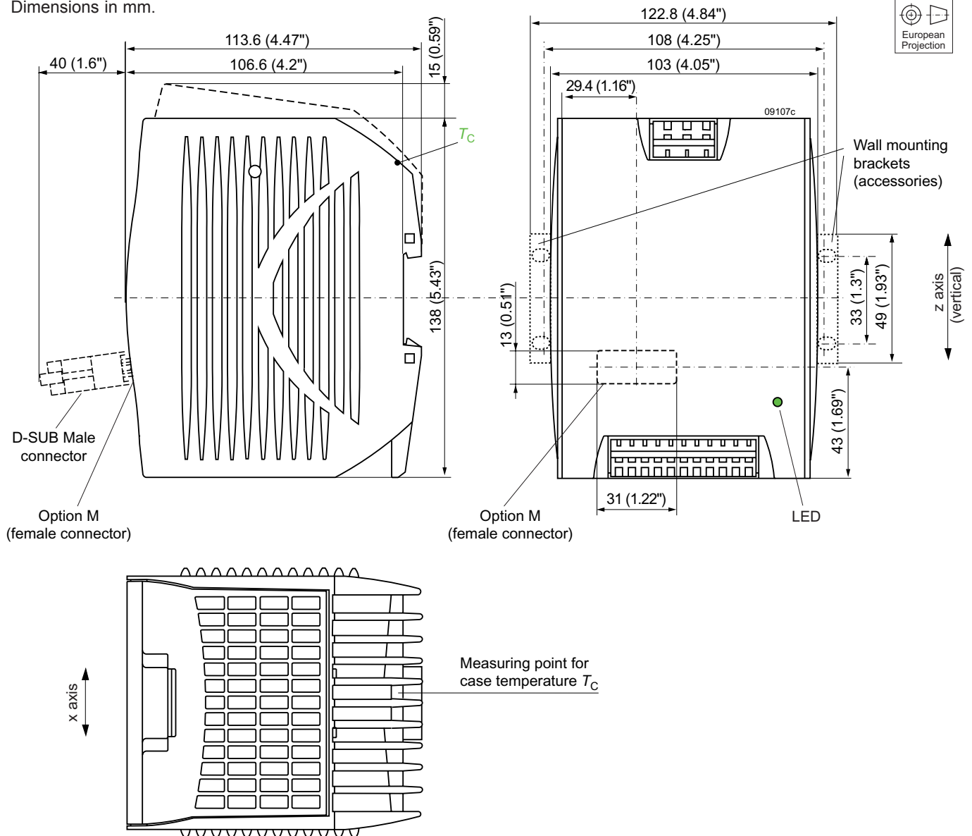
Fig. 16 Case W01 EWN/LWN: weight approx. 1400 g EWL/LWR: weight approx. 1200 g Case designed by ATP, Munich.
