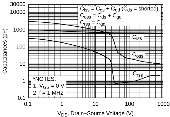
Figure 5. Capacitance Characteristics
