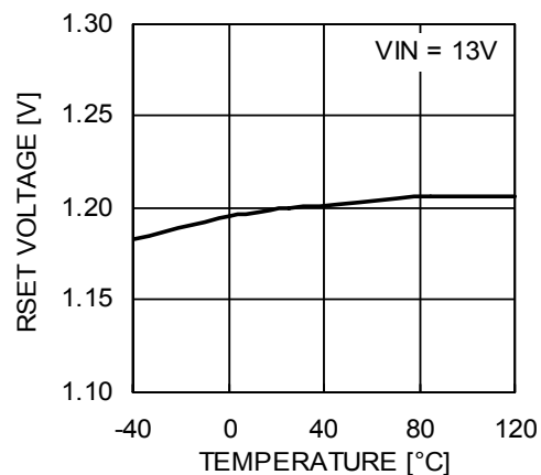
RSET Voltage vs. Temperature
