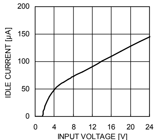
Idle Mode Supply Current (CTRL = 0V)
