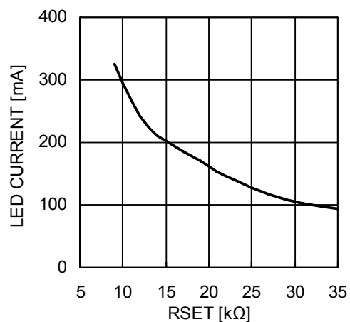
LED Current vs. RSET
