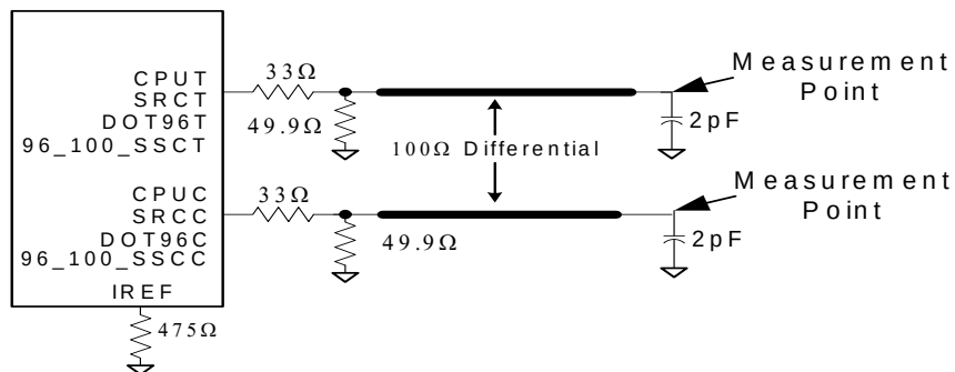
Figure 15. 0.7V Differential Load Configuration
