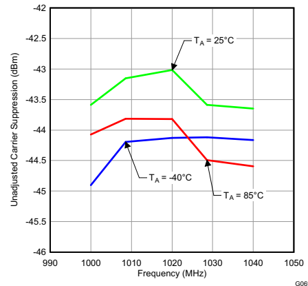
Figure 72. Unadjusted Carrier Suppression vs Frequency and Temperature at 1030 MHz
