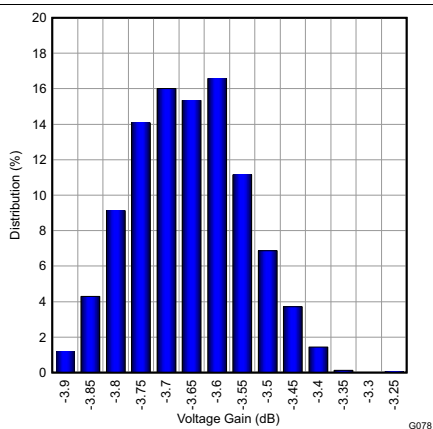
Figure 90. Gain at 2300-MHz Distribution
