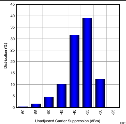
Figure 93. Unadjusted Carrier Suppression at 2300-MHz Distribution
