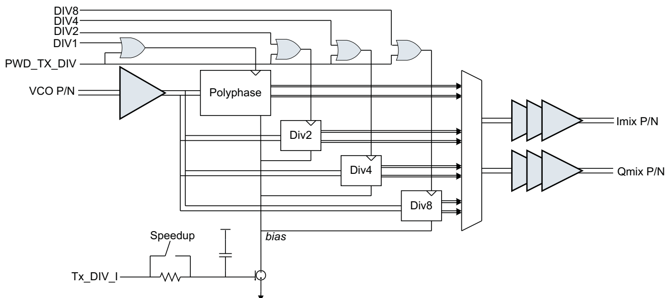
Figure 80. Tx Divider
