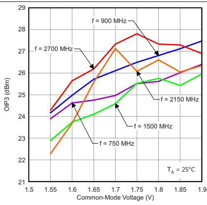
Figure 55. OIP3 vs Common-Mode Voltage and Frequency
