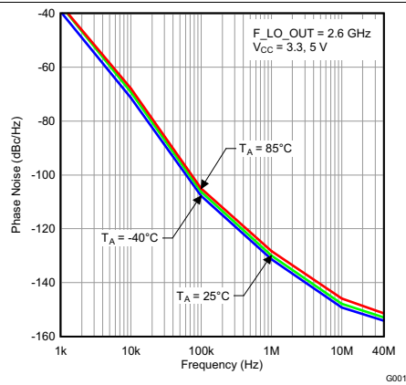
Figure 3. Open-Loop Phase Noise vs Frequency and Temperature
