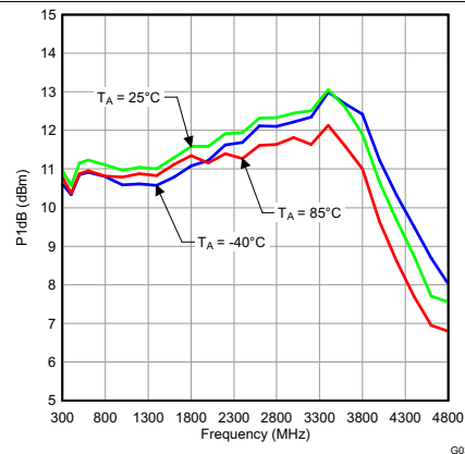
Figure 41. P1dB vs Frequency and Temperature
