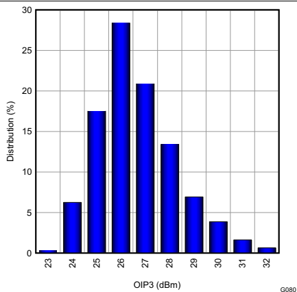
Figure 92. OIP3 at 2300-MHz Distribution
