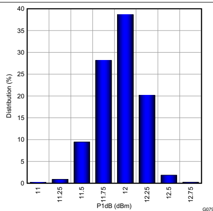
Figure 91. P1dB at 2300-MHz Distribution
