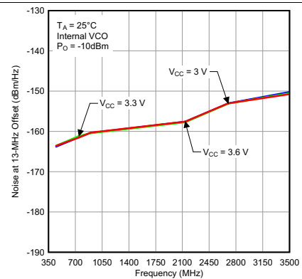
Figure 28. Noise at 13-MHz Offset vs Frequency and Supply Voltage With Internal VCO
