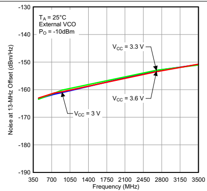
Figure 30. Noise at 13-MHz Offset vs Frequency and Supply Voltage With External VCO
