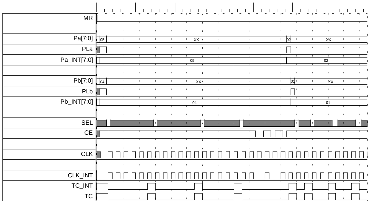
Figure 10. Device Timing Diagram for Table 12
