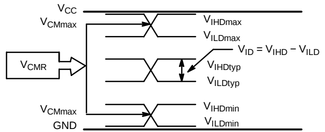
Figure 22. V_{CM} Diagram
