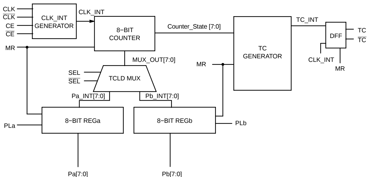
Figure 4. Block Diagram
