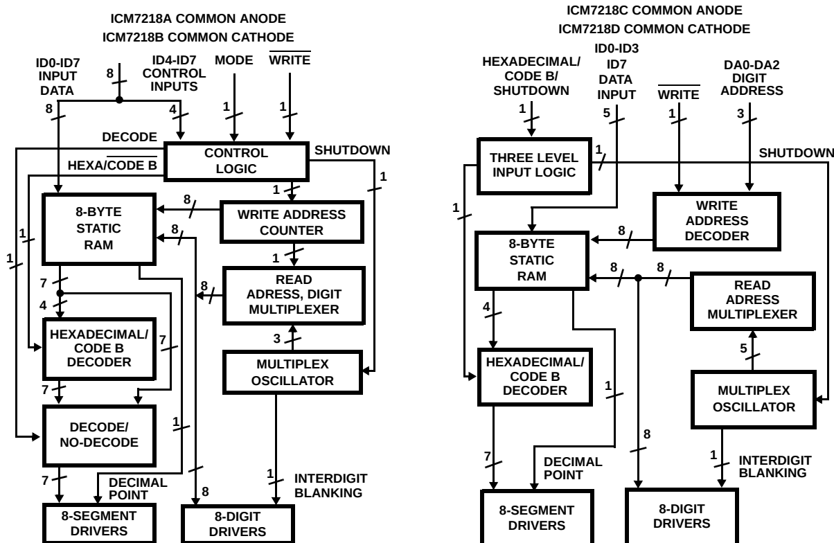
FIGURE 1. FUNCTIONAL DIAGRAMS
