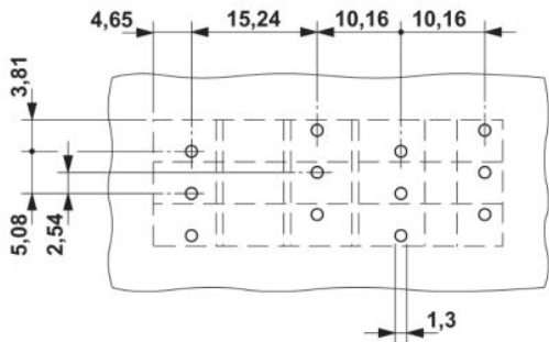
Drilling plan/solder pad geometry
