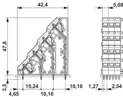
Dimensioned drawing
