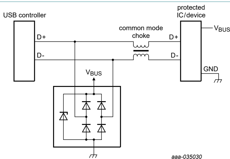
Fig. 5. Application diagram: USB 2.0
