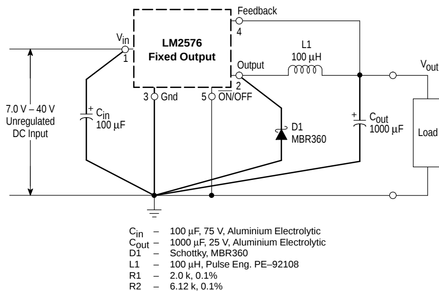
Figure 15. Typical Test Circuit
