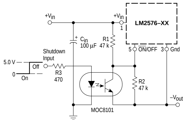
Figure 28. Inverting Buck–Boost Regulator Shutdown Circuit Using an Optocoupler
