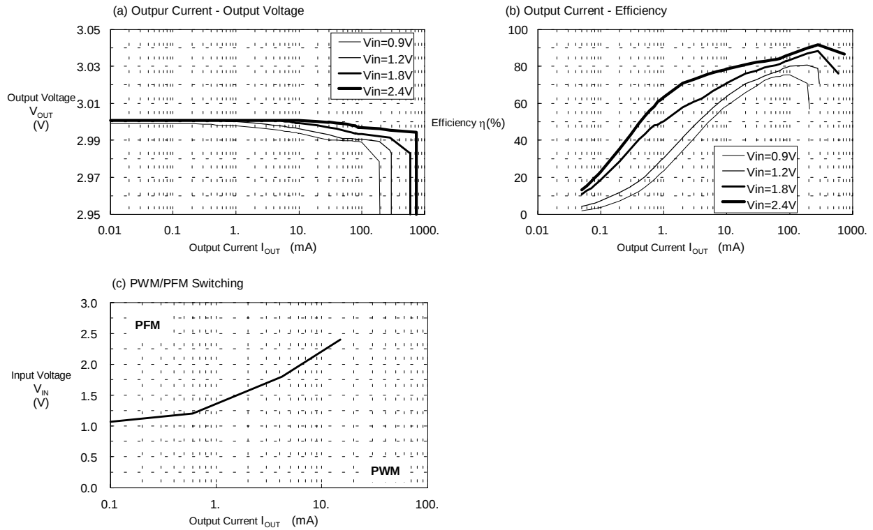
(11) S-8328B30 (CD105 : 22 \mu H, Rb=1k \Omega , Cb=0.0022 \mu F)
