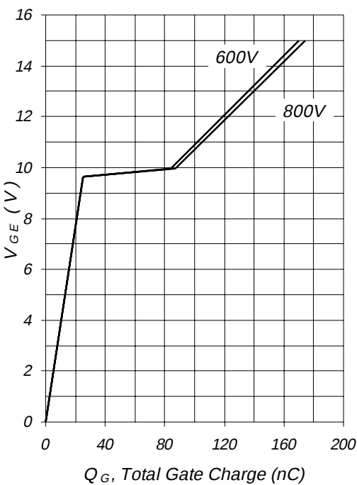
Fig.23 - Typ. Gate Charge vs. V_{GE} I_C=20\text{A} ; L=600\mu\text{H}
