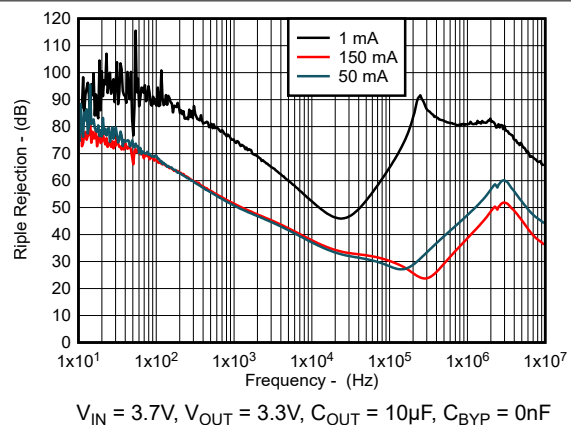
Figure 5-14. Ripple Rejection vs Frequency (New Chip)
