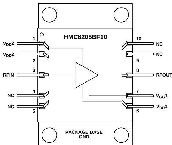
Figure 2. Pin Configuration
