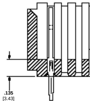
Detail E
