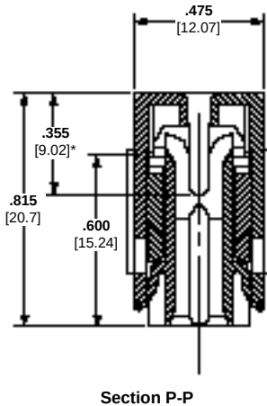
Section P-P
