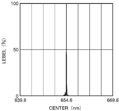
Fig.3 Emission spectrum
