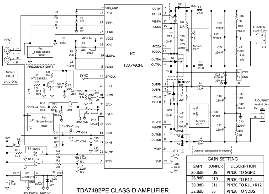
Figure 7. Application circuit
