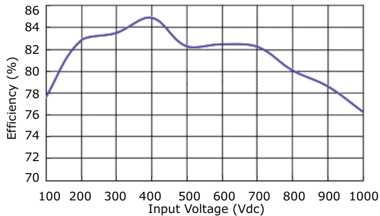
AE10-EW-S24 Efficiency Curve Efficiency vs. Input Voltage
