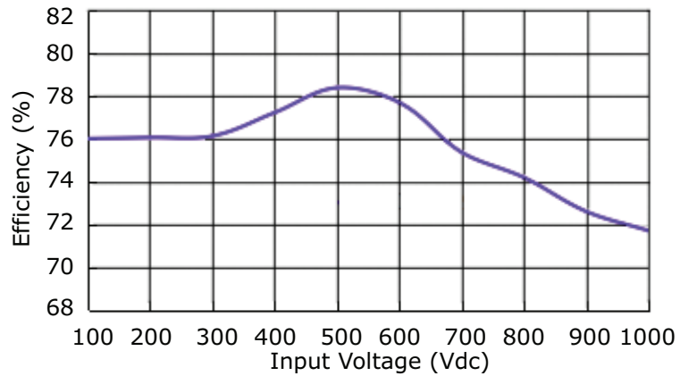
AE10-EW-S9 Efficiency Curve Efficiency vs. Input Voltage
