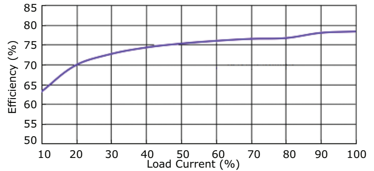
AE10-EW-S9 Efficiency Curve Efficiency vs. Load Current
