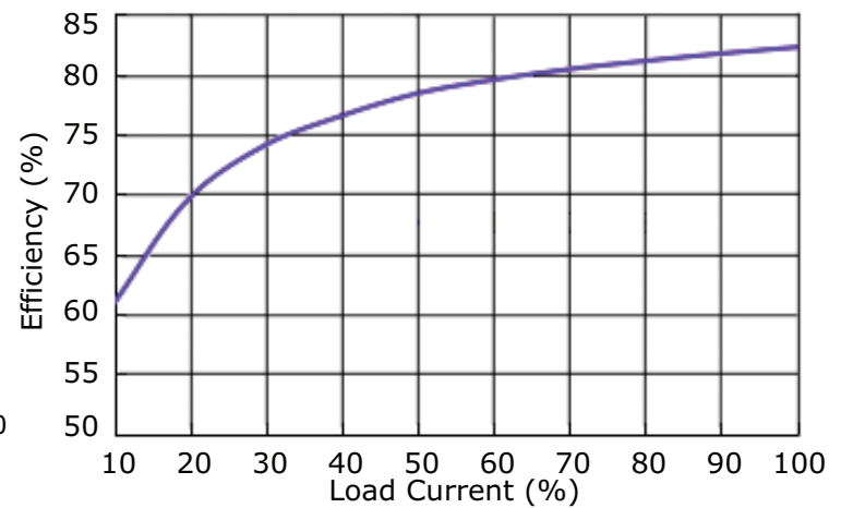
AE10-EW-S24 Efficiency Curve Efficiency vs. Load Current
