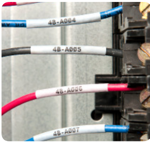
Self-Laminating Wire & Cable Markers
