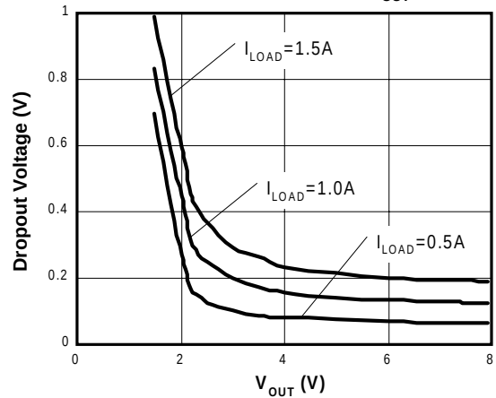
Dropout Voltage vs. V_{OUT}
