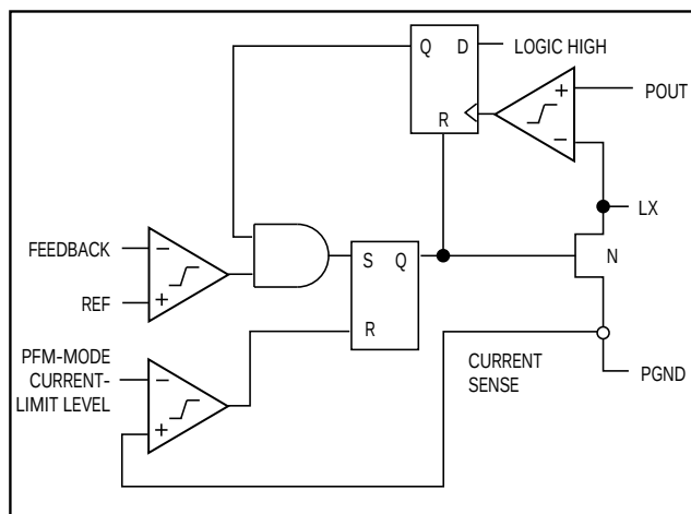
Figure 3. Controller Block Diagram in PFM Mode
