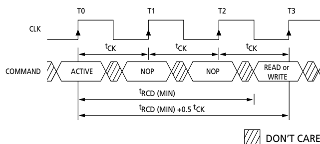
Figure 7: Example: Meeting t_{RCD}(\text{MIN}) When 2 < t_{RCD}(\text{MIN})/t_{CK} - 3
