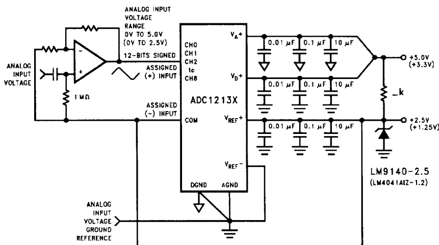
FIGURE 11. Alternative Pseudo-Differential Biasing
