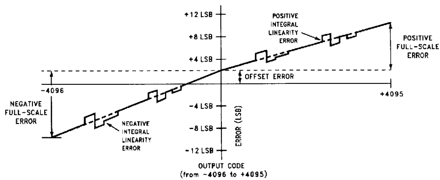
FIGURE 1b. Simplified Error Curve vs Output Code without Auto-Calibration or Auto-Zero Cycles
