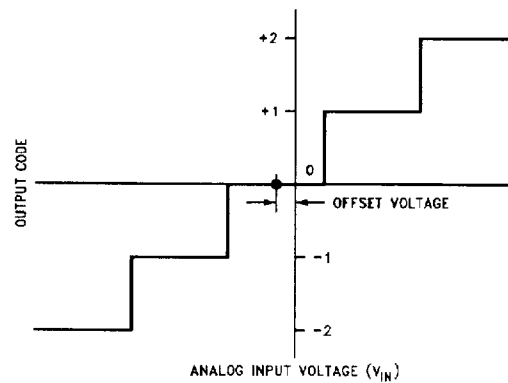
FIGURE 2. Offset or Zero Error Voltage
