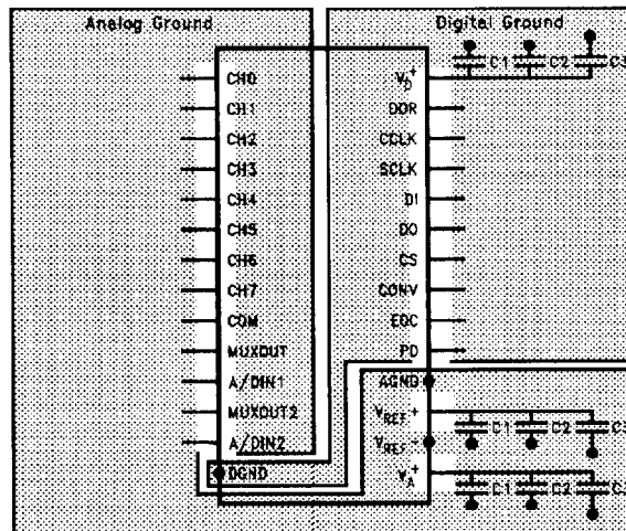
FIGURE 16. Ideal Ground Plane
