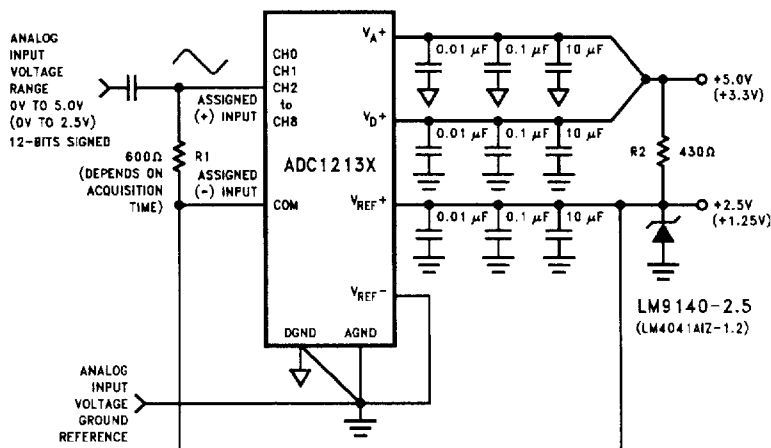
FIGURE 10. Pseudo-Differential Biasing with the Signal Source AC Coupled Directly Into the ADC
