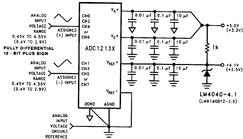
FIGURE 13. Fully Differential Biasing
