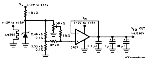
FIGURE 14. Low Drift Extremely Stable Reference Circuit
