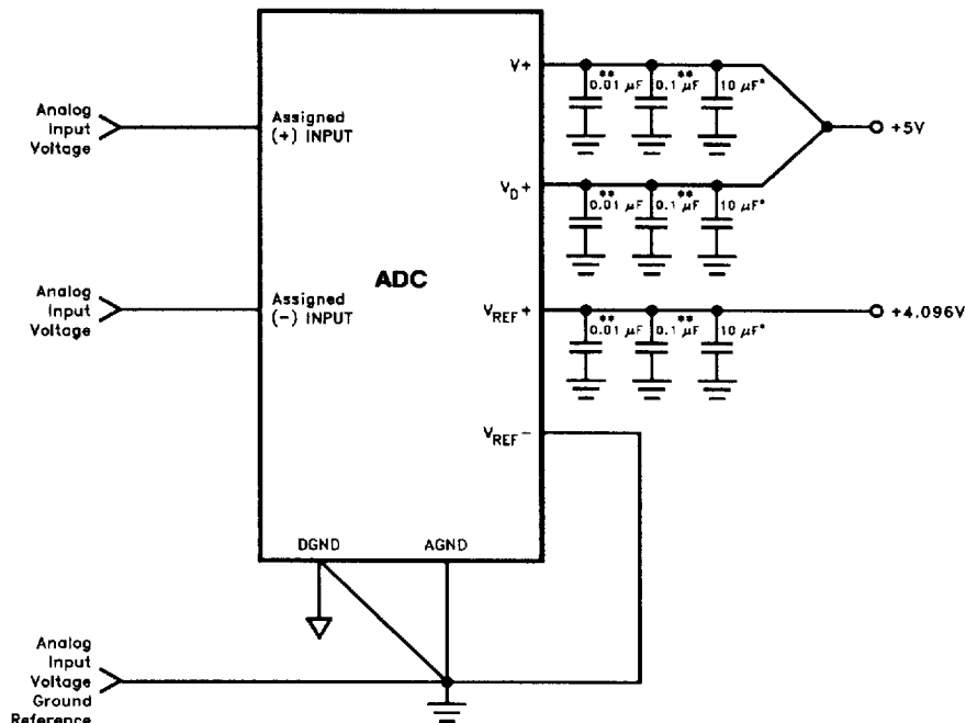
FIGURE 4. Recommended Power Supply Bypassing and Grounding
