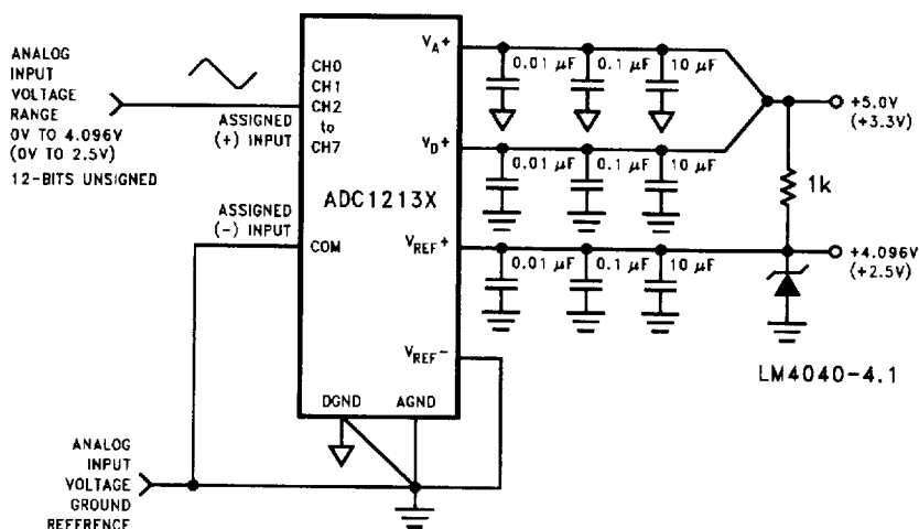
FIGURE 9. Single-Ended Biasing
