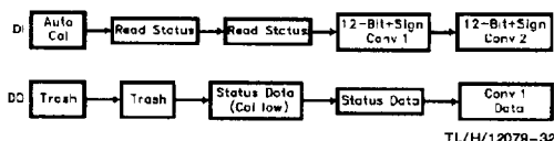
FIGURE 5. Typical Power Supply Power Up Sequence
