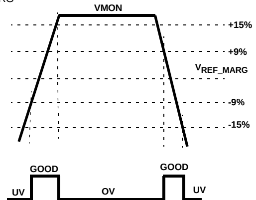
FIGURE 3. UNDERVOLTAGE-OVERVOLTAGE WINDOW
