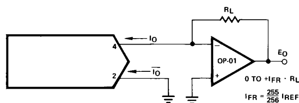
Figure 26. Positive Low Impedance Output Operation
