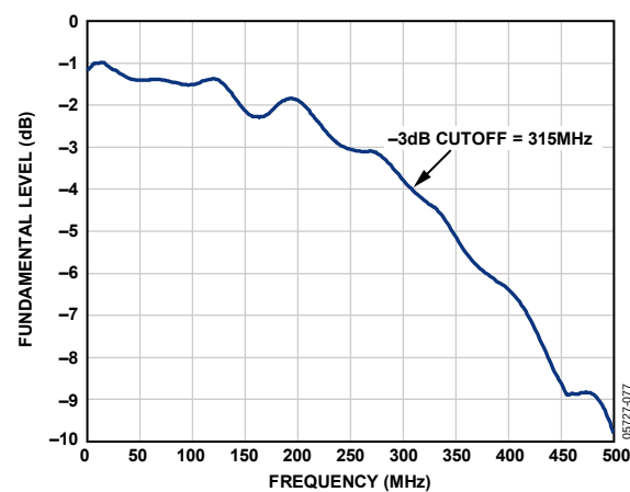
Figure 42. Full-Power Bandwidth vs. Frequency, f_{\text{SAMPLE}} = 65 \text{ MSPS}
